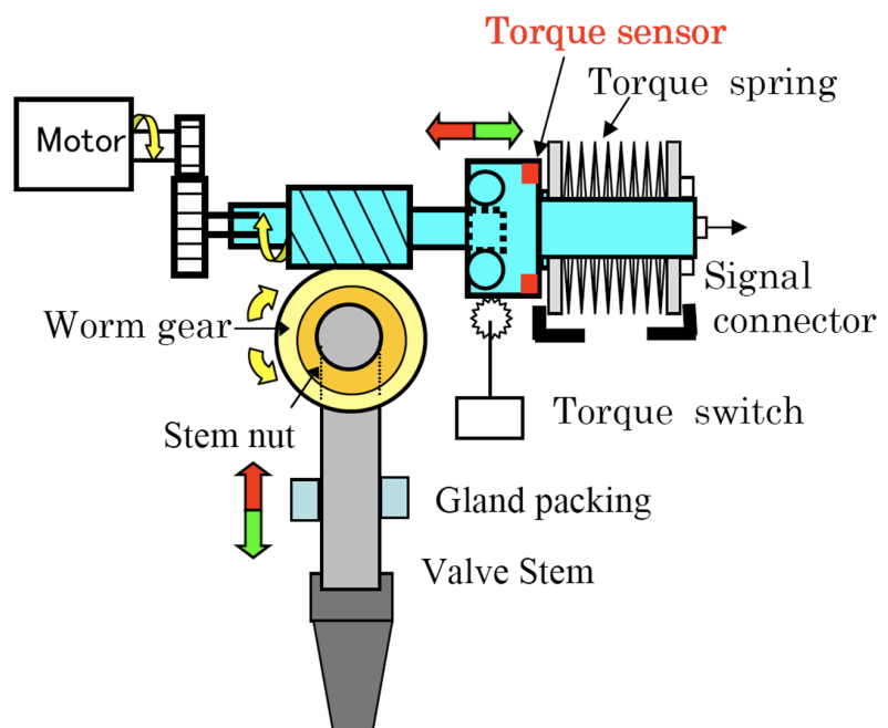
Basic MOV design with torque sensor
